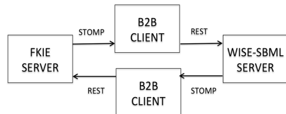
Figure 4. Two-Servers Interconnected With Back-to-back Clients
